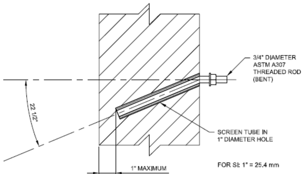
FIGURE 2—HILTI HIT-HY 270 ADHESIVE 22½° COMBINATION ANCHOR (CONFIGURATION B)
